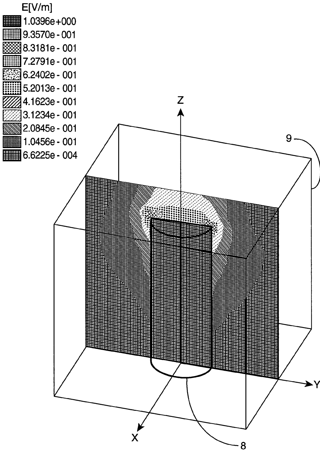
FIG. 1C PRIOR ART
